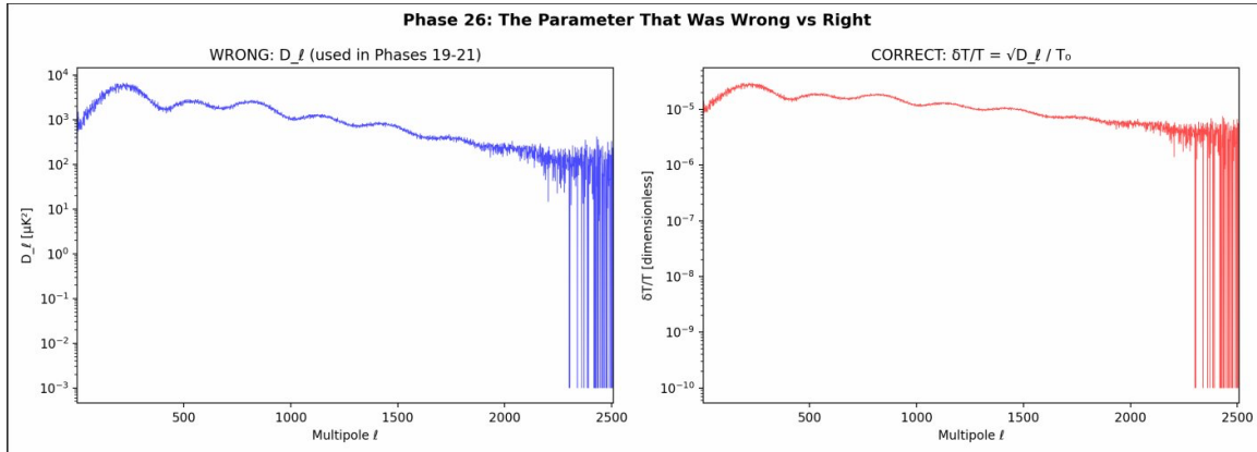
Figure 2. The CMB normalisation correction (Phase 26). Left: the originally used D_\ell power spectrum — incorrect for cross-substrate comparison due to the \ell(\ell+1)/2\pi weighting. Right: the corrected \delta T/T = \sqrt{D_\ell}/T_0 (dimensionless temperature fluctuations). The correction was identified and implemented during Phase 26. All CMB cross-substrate results reported in Section 3.3 use the corrected \delta T/T normalisation.
