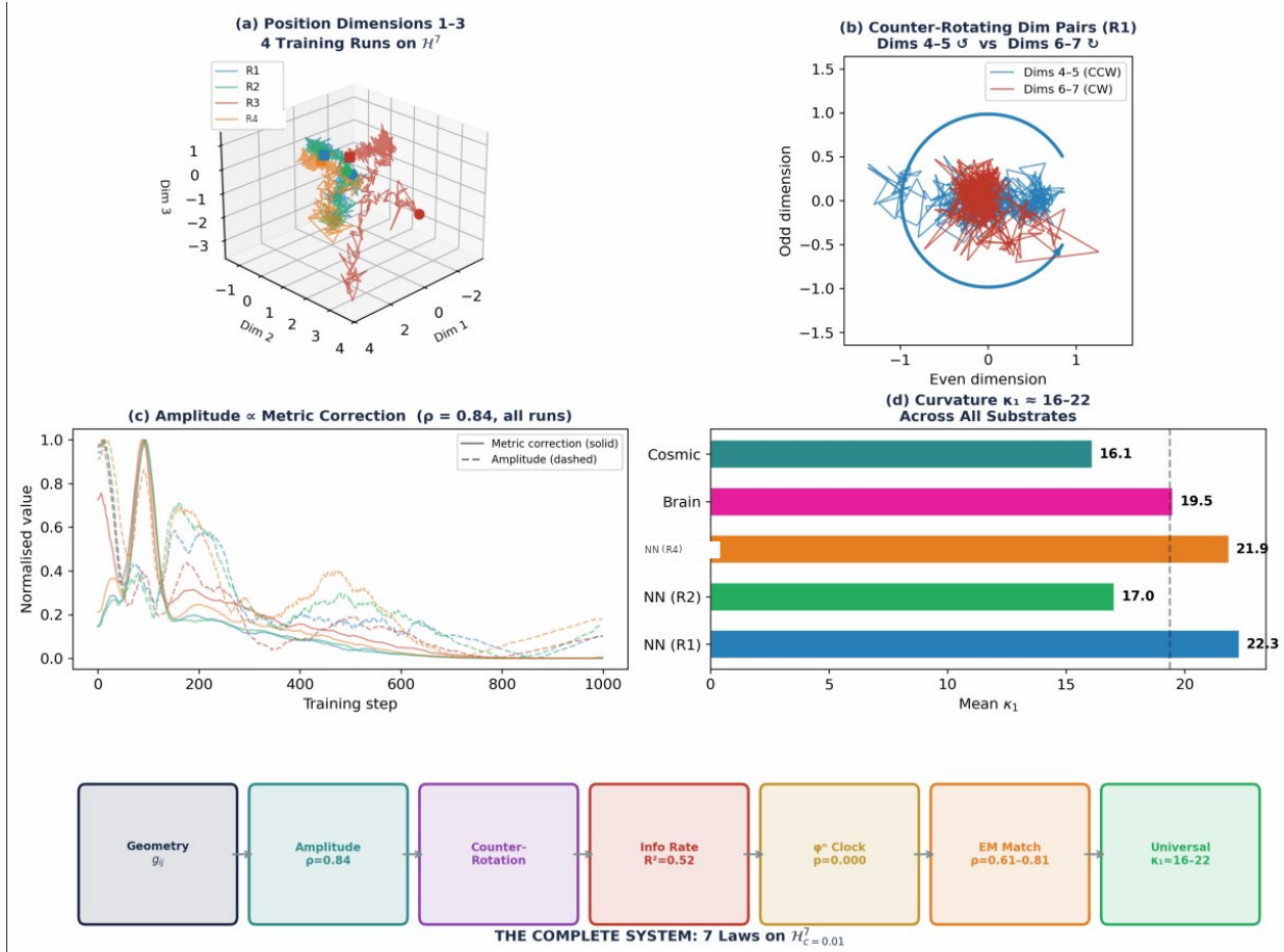
Figure 5. The seven laws of the H^7 manifold. (a) Position dimensions 1–3: trajectories of all four training runs in 3D projection of H^7 . R3 (perturbed) diverges from the attractor basin reached by R1 , R2 , and R4 . (b) Counter-rotating dimension pairs in R1 : dims 4–5 rotate CCW (blue) while dims 6–7 rotate CW (red) — opposite chirality confirmed across all control runs. (c) Amplitude \propto metric correction, \rho=0.84 across all runs. (d) Curvature \kappa_i \approx 16-22 is substrate-invariant across Cosmic, Brain, and all NN control runs. Bottom: the complete 7-law chain governing H^7 geometry.
