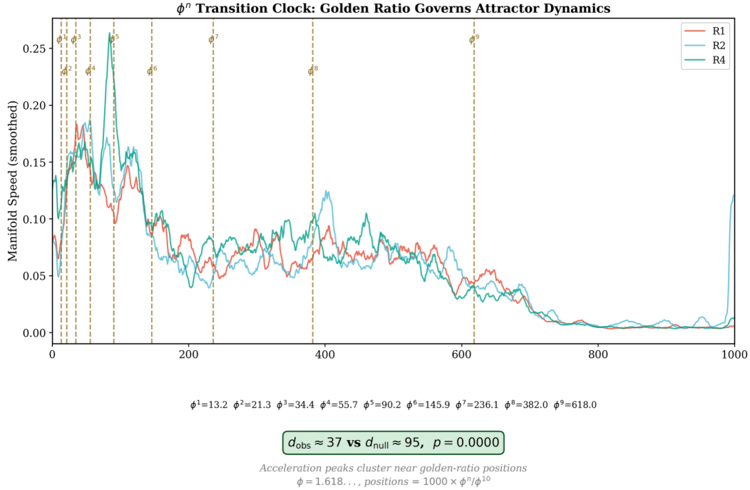
Figure 14. The \phi^n transition clock. Manifold speed (smoothed) across 1,000 training steps for three control runs (R1, R2, R4). Dashed vertical lines mark golden-ratio positions s_n = \phi^n / \phi^{10} \times 1000 ( n = 1, \dots, 9 ). Acceleration peaks cluster near these positions: d_{\text{obs}} \sim 37 steps vs d_{\text{null}} \sim 95 steps (10,000 permutations), p < 0.0001 across all four runs. R3 also confirms ( p < 0.0001 ) but is omitted for visual clarity; see Section 3.1.
