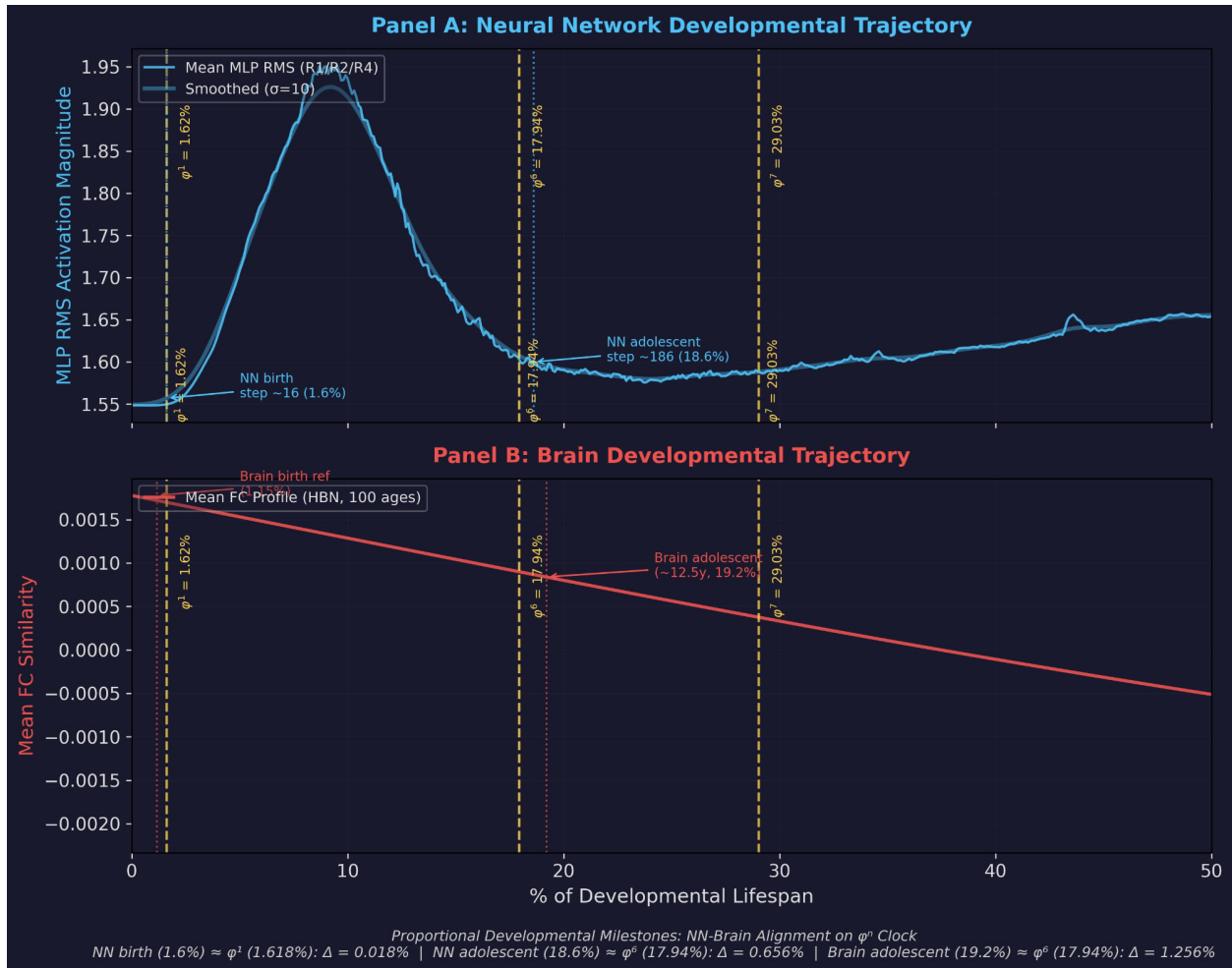
Figure 18. Proportional developmental milestones: NN-Brain alignment on the \phi^n clock. Panel A: Mean MLP RMS activation magnitude across training steps for R1/R2/R4 (raw and smoothed \sigma=10 ). Two structural events are marked: organisational onset at step ~16 (1.6% of training) and adolescent reorganisation dip at step ~186 (18.6%). Panel B: Mean FC similarity profile (HBN cohort, 100 age bins) across developmental lifespan, normalised to % of lifespan. Brain birth reference at 1.15% and adolescent FC inversion at ~12.5y (19.2% of lifespan; note: distinct from the collective gradient sign reversal at 14.93–15.79y in Section 3.8, which tests a different feature of adolescent reorganisation) are marked. Gold dashed vertical lines in both panels: \phi^1=1.618\% , \phi^6=17.94\% , \phi^7=29.03\% . Proportional alignment: NN birth 1.6% \approx \phi^1 1.618% ( \Delta=0.018\% ); NN adolescent 18.6% \approx \phi^6 17.94% ( \Delta=0.656\% ); Brain adolescent 19.2% \approx \phi^6 17.94% ( \Delta=1.256\% ). Eight independent measurements (4 NN runs \times 4 brain cohorts). Joint p=0.019 .
