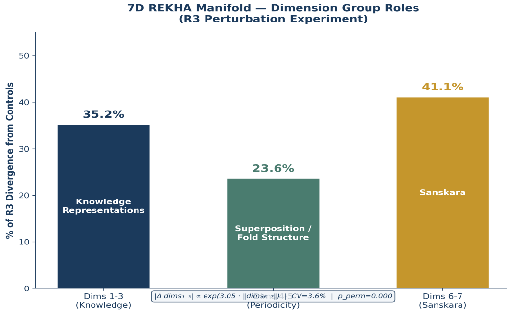
Figure 11. Seven-dimensional attractor decomposition from the R3 perturbation experiment. Dims 6–7 (Sanskara) account for 41.1% of attractor divergence despite carrying only 8.2% of total variance — a 5.01 \times amplification. The exponential coupling equation (Eq. 8) is shown. Dims 1–3 = Knowledge Representations; Dims 4–5 = Superposition/Fold Structure; Dims 6–7 = Sanskara.
