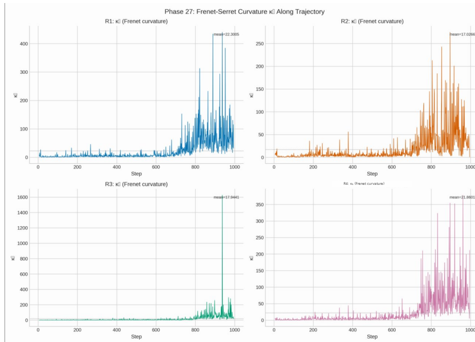
Figure 4. Frenet–Serret principal curvature \kappa_1 along the training trajectory for all four runs (Phase 27). Mean
