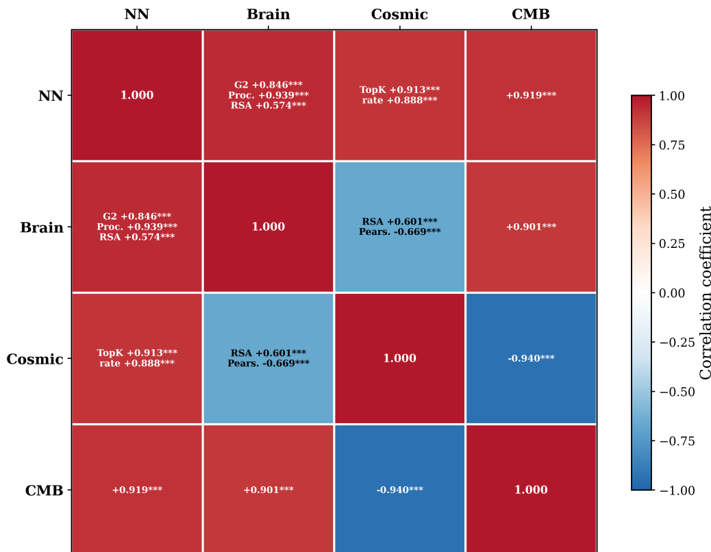
Figure 7. Cross-substrate depth profile correlation matrix. All pairwise correlations computed via Spearman rank correlation with permutation null testing (10,000 permutations). All reported values significant at p < 0.001 . NN = SWARAJ neural network; Brain = HCP functional connectivity gradients; Cosmic = THESAN/DisPerSE filament density; CMB = Planck temperature fluctuations.
