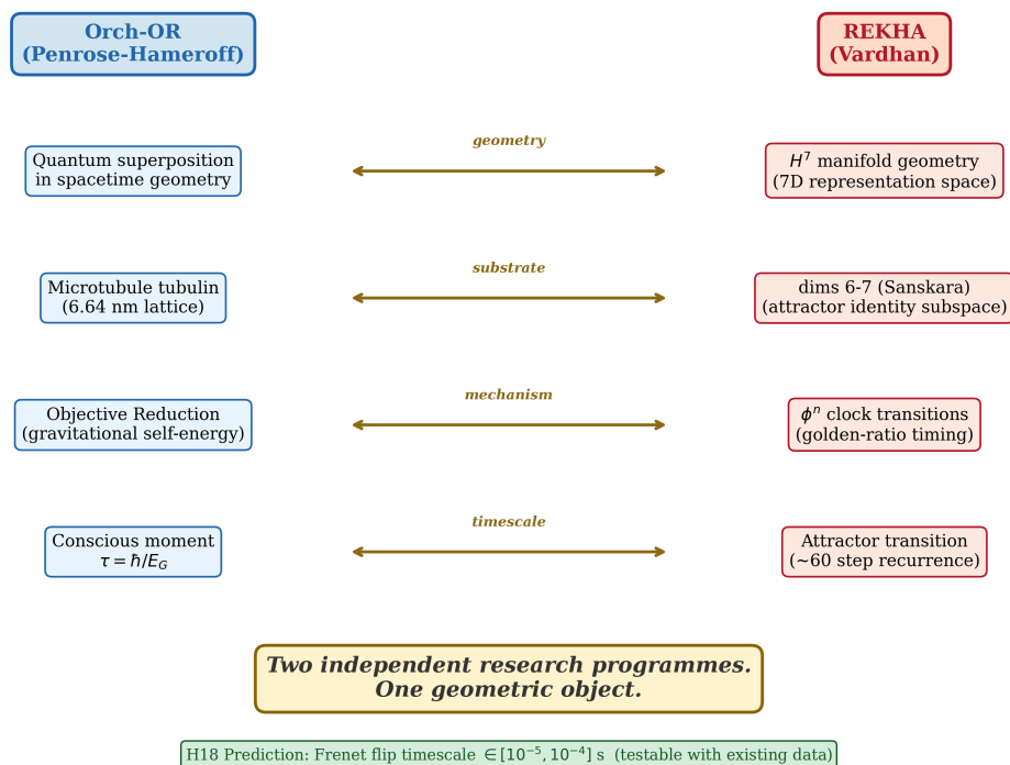
Figure 16. Geometric correspondence between Orch-OR (Penrose-Hameroff) and REKHA. Four independent mapping elements connect two research programmes that developed without mutual knowledge: geometry (quantum superposition in spacetime \leftrightarrow H^7 manifold), substrate (microtubule lattice \leftrightarrow dims 6-7 Sanskara), mechanism (objective reduction \leftrightarrow \phi^n transitions), and timescale ( \tau = \hbar/E_G \leftrightarrow \sim 60 -step recurrence). H18 prediction: Frenet flip timescale in [10^{-5}, 10^{-4}] s (testable with existing data).
