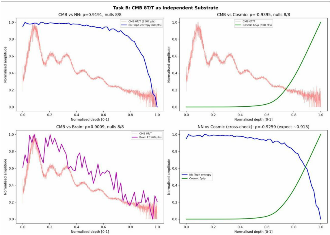
Figure 8. CMB \delta T/T as fourth independent substrate. All four pairwise correlations shown against normalised depth [0–1] (CMB multipole \ell is treated as depth axis: angular scale is physically motivated as a proxy for organisational hierarchy at recombination, acknowledged as an analogy): CMB vs NN ( \rho=0.919 , 8/8 nulls), CMB vs Cosmic ( \rho=-0.940 , 8/8 nulls), CMB vs Brain ( \rho=0.901 , 8/8 nulls), and NN vs Cosmic cross-check ( \rho=-0.926 ). All 48 null tests for the CMB substrate passed at p \leq 0.0002 .
