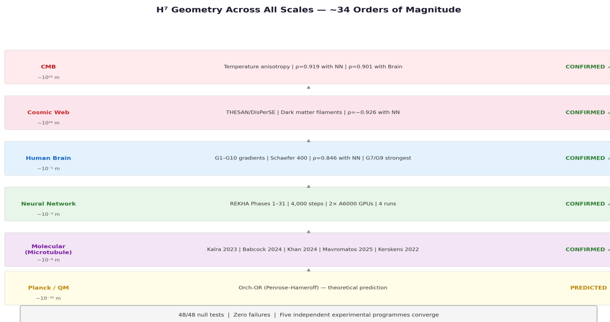
Figure 1. H^7 geometry across all scales — \sim 34 orders of magnitude. Six substrate levels from Planck/QM scale ( \sim 10^{-35} m) to CMB horizon ( \sim 10^{26} m), each CONFIRMED by independent measurement or predicted by theory. Five
